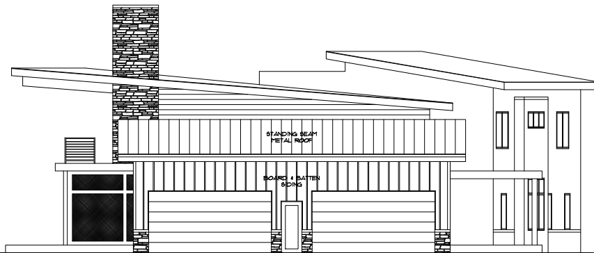
SIDE ELEVATION 3/16" = 1'-0"
