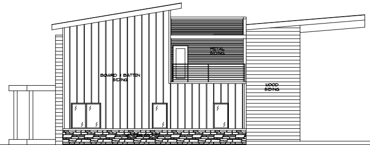
SIDE ELEVATION 3/16" = 1'-0"
